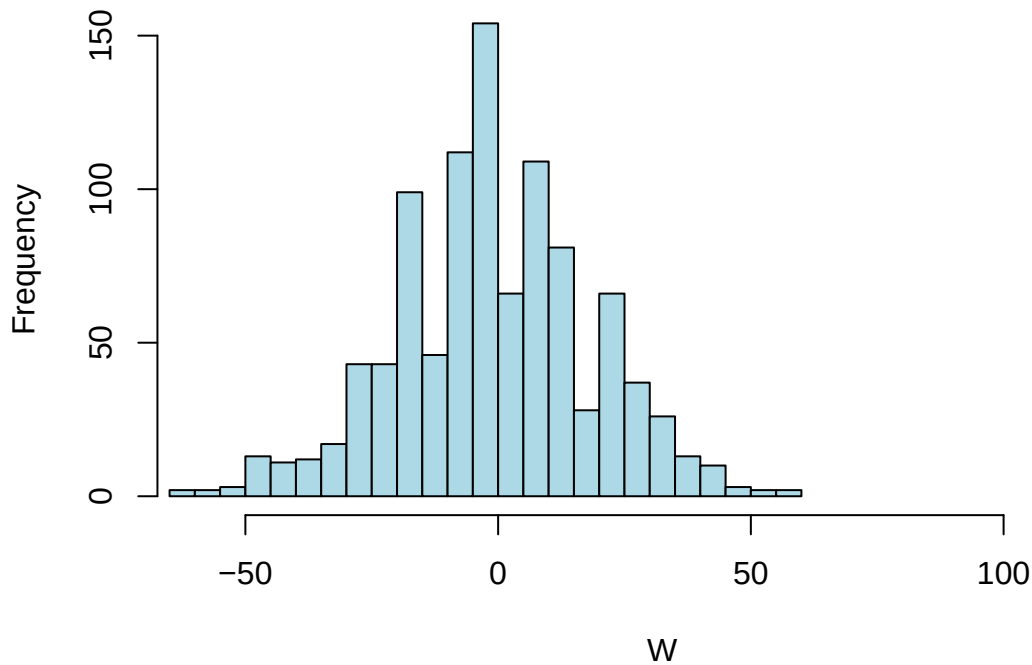
Histogram of simulated W^* values under null
